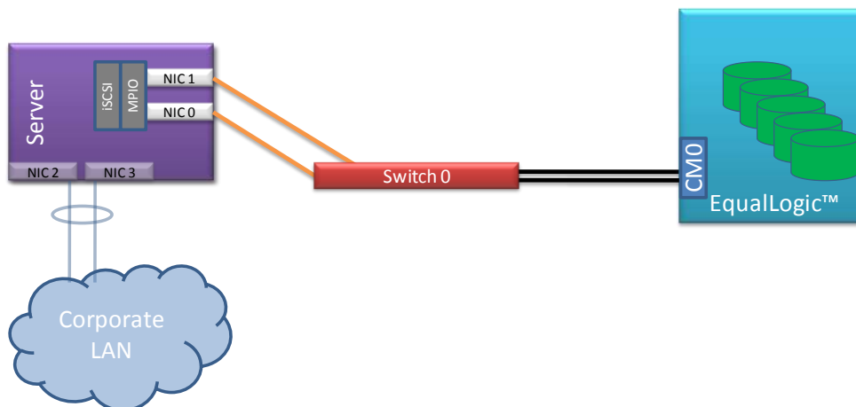
Figure 12: Single Switch/Dual NIC
