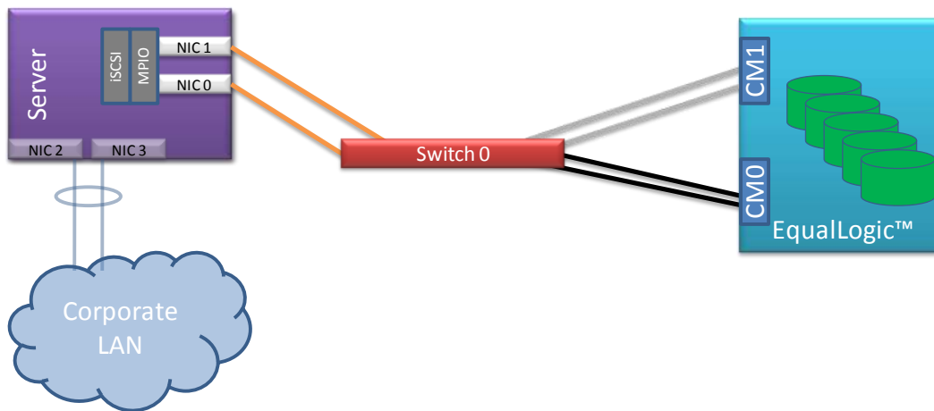
Figure 16: Single Switch/Dual NIC
