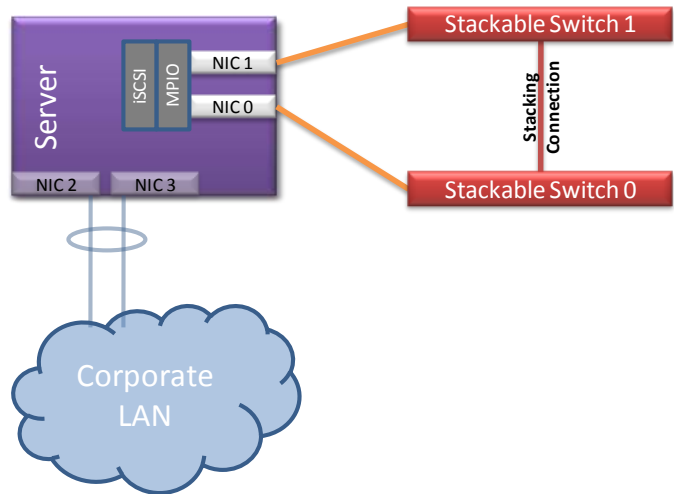
Figure 7: Single Controller Array to Switch Configuration
