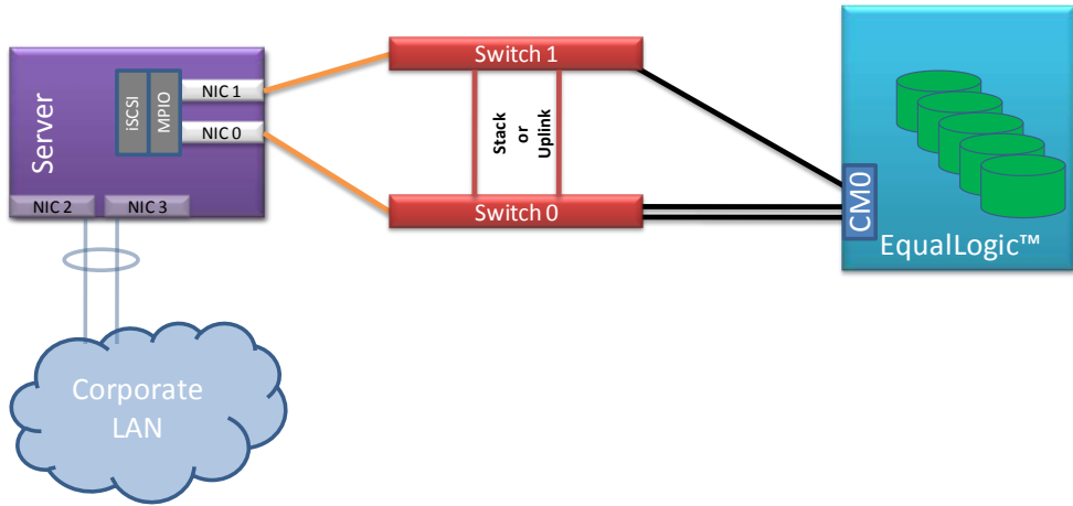
Figure 13: Dual Switch/Dual NIC
