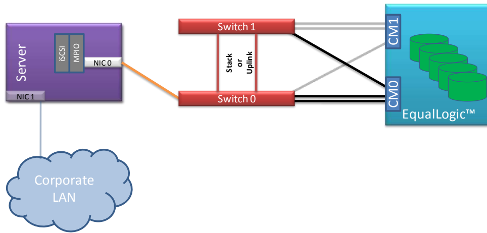
Figure 15: Dual Switch/Single NIC
