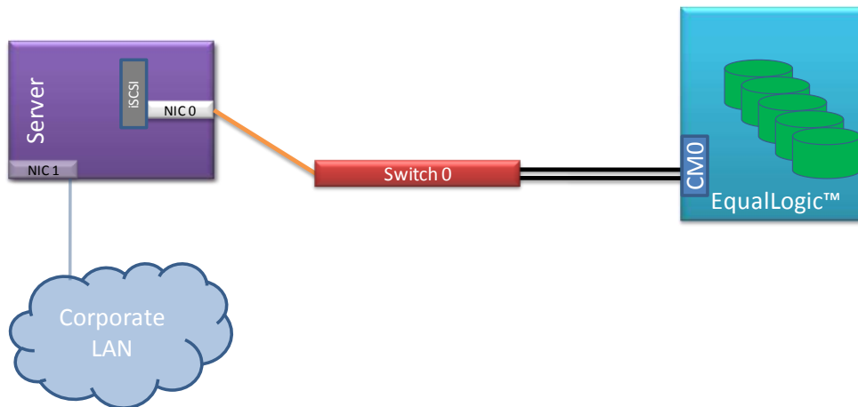
Figure 11: Single Switch/Single NIC
